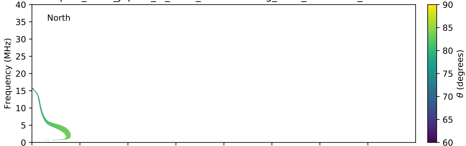
expres_earth_jupiter_io_isaac_lossc-wid1deg_3kev_20170615_v01.cdf
