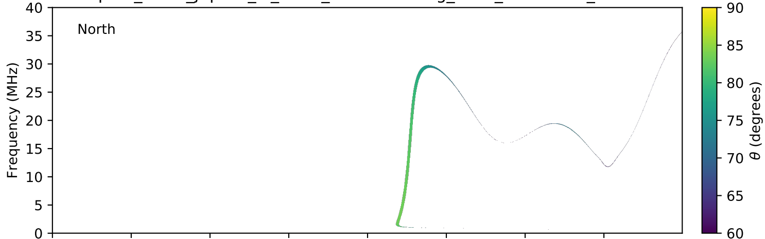
expres_earth_jupiter_io_isaac_lossc-wid1deg_3kev_20170612_v01.cdf
