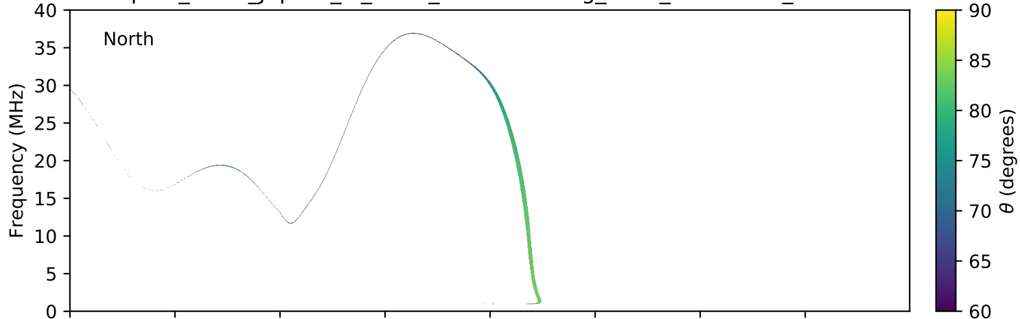
expres_earth_jupiter_io_isaac_lossc-wid1deg_3kev_20170611_v01.cdf
