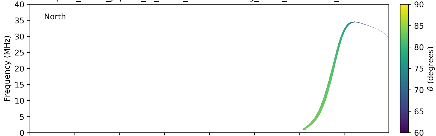
expres_earth_jupiter_io_isaac_lossc-wid1deg_3kev_20170610_v01.cdf
