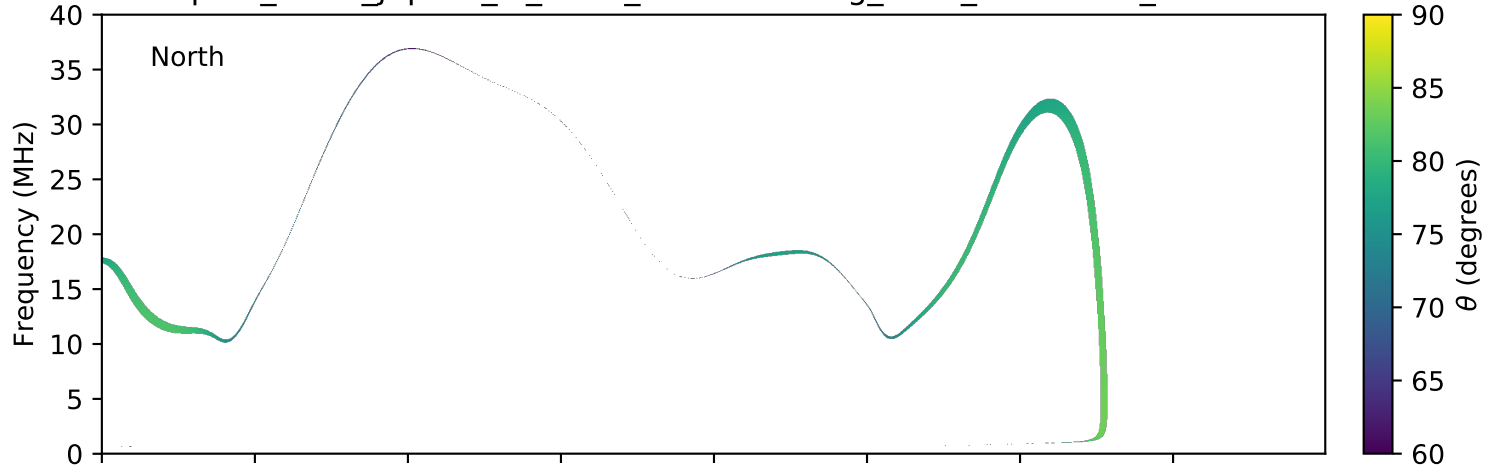
expres_earth_jupiter_io_isaac_lossc-wid1deg_3kev_20170609_v01.cdf
