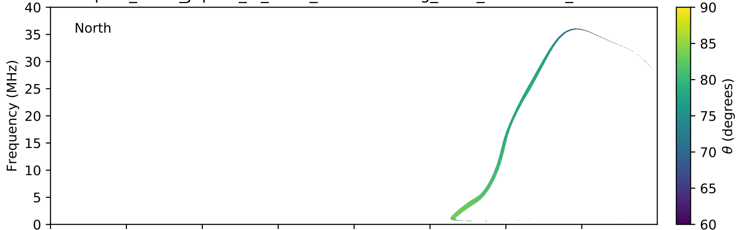
expres_earth_jupiter_io_isaac_lossc-wid1deg_3kev_20170603_v01.cdf
