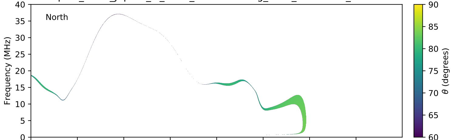
expres_earth_jupiter_io_isaac_lossc-wid1deg_3kev_20170602_v01.cdf
