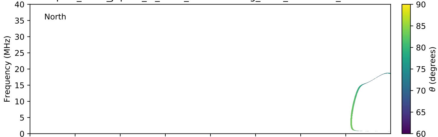
expres_earth_jupiter_io_isaac_lossc-wid1deg_3kev_20170601_v01.cdf
