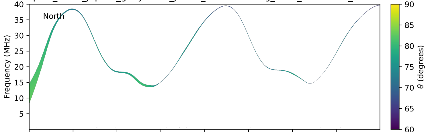
expres_earth_jupiter_ganymede_jrm33_lossc-wid1deg_3kev_20170610_v11.cdf
