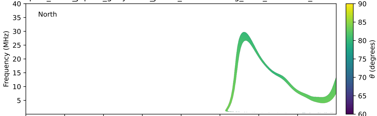
expres_earth_jupiter_ganymede_jrm33_lossc-wid1deg_3kev_20170609_v11.cdf
