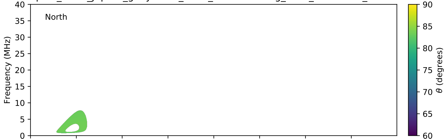
expres_earth_jupiter_ganymede_isaac_lossc-wid1deg_3kev_20170627_v01.cdf
