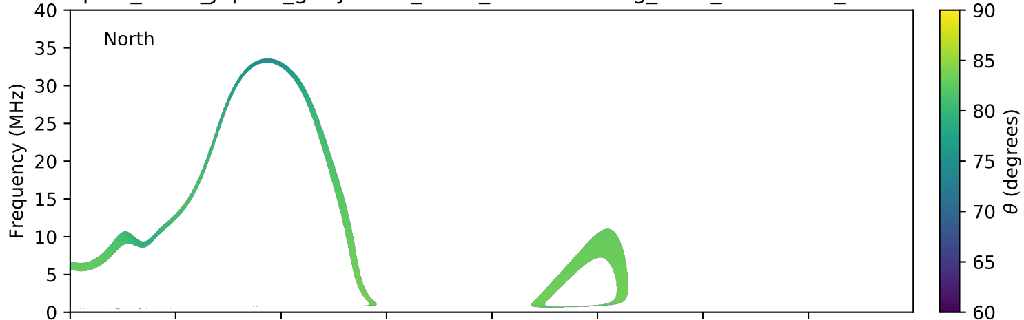
expres_earth_jupiter_ganymede_isaac_lossc-wid1deg_3kev_20170605_v01.cdf
