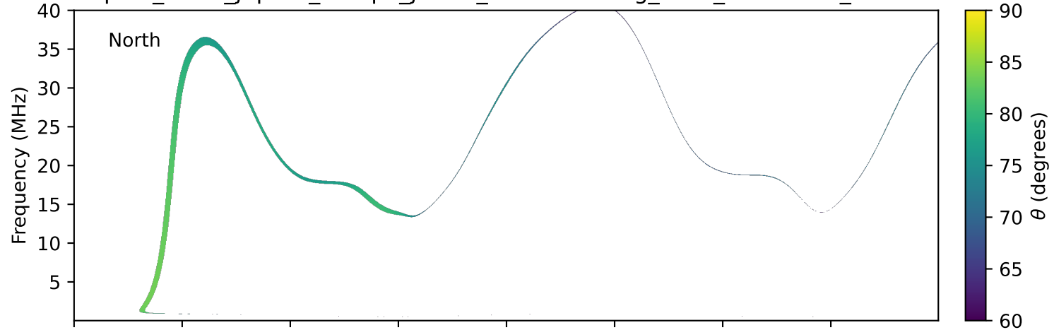
expres_earth_jupiter_europa_jrm33_lossc-wid1deg_3kev_20170605_v11.cdf
