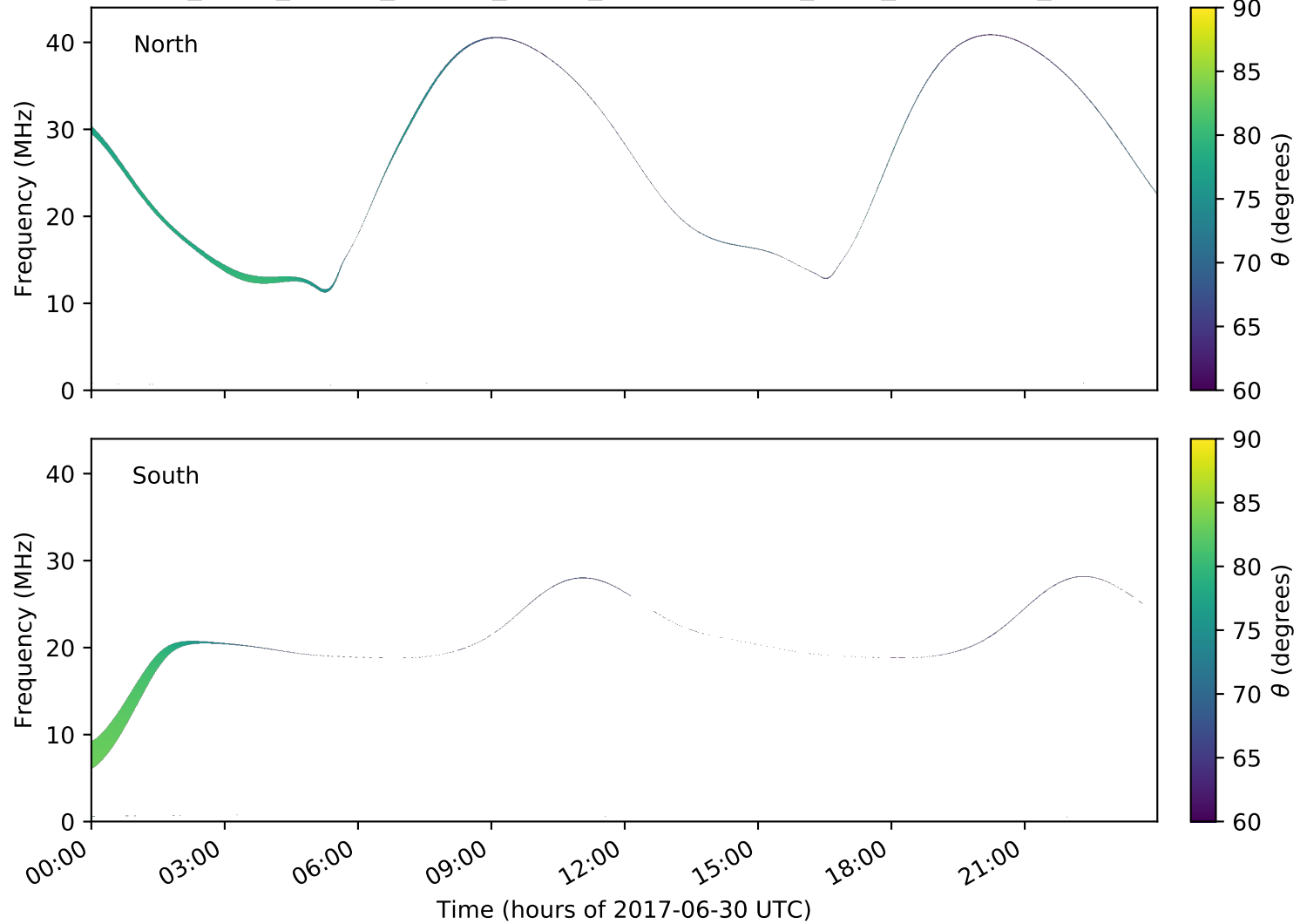
expres_earth_jupiter_europa_jrm09_lossc-wid1deg_3kev_20170630_v01.cdf
