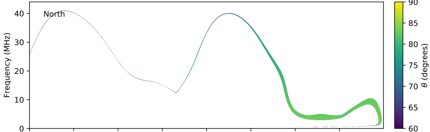
expres_earth_jupiter_europa_jrm09_lossc-wid1deg_3kev_20170627_v01.cdf
