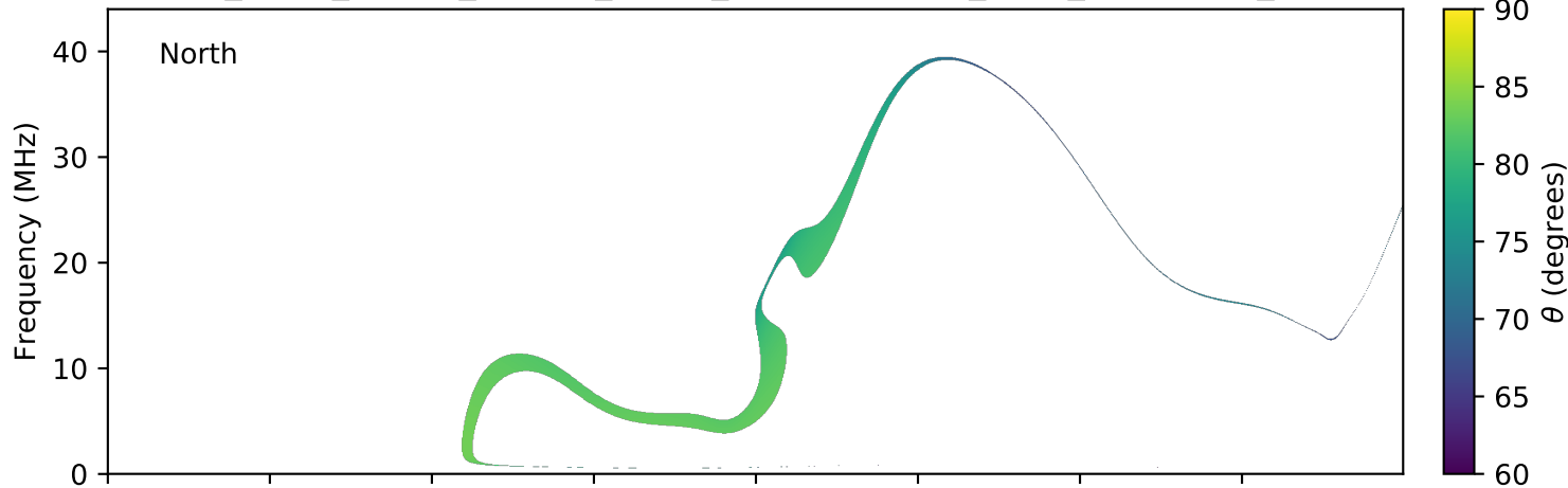
expres_earth_jupiter_europa_jrm09_lossc-wid1deg_3kev_20170626_v01.cdf
