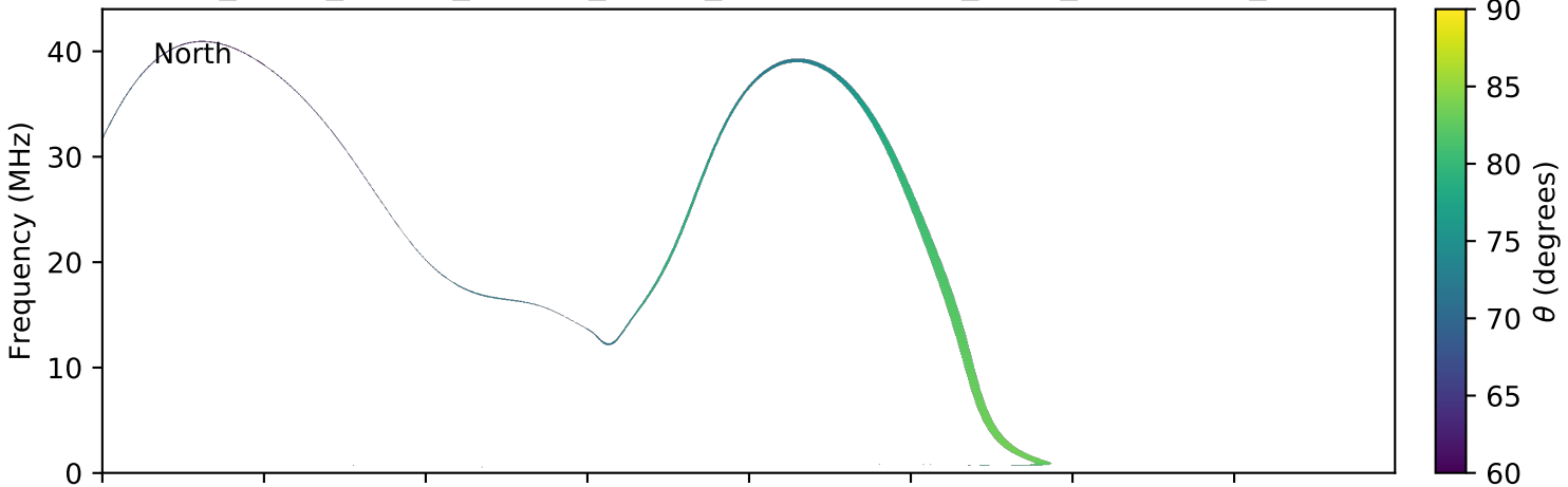
expres_earth_jupiter_europa_jrm09_lossc-wid1deg_3kev_20170620_v01.cdf
