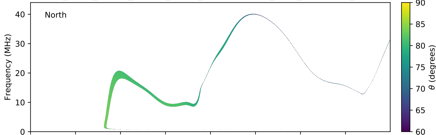
expres_earth_jupiter_europa_jrm09_lossc-wid1deg_3kev_20170619_v01.cdf
