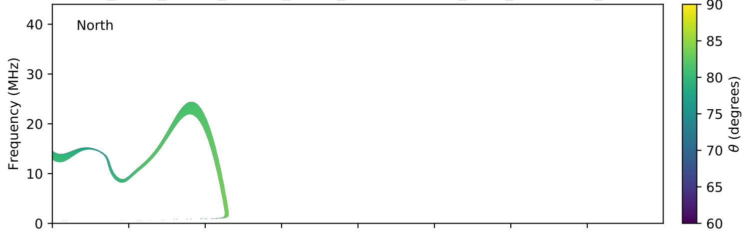
expres_earth_jupiter_europa_jrm09_lossc-wid1deg_3kev_20170617_v01.cdf
