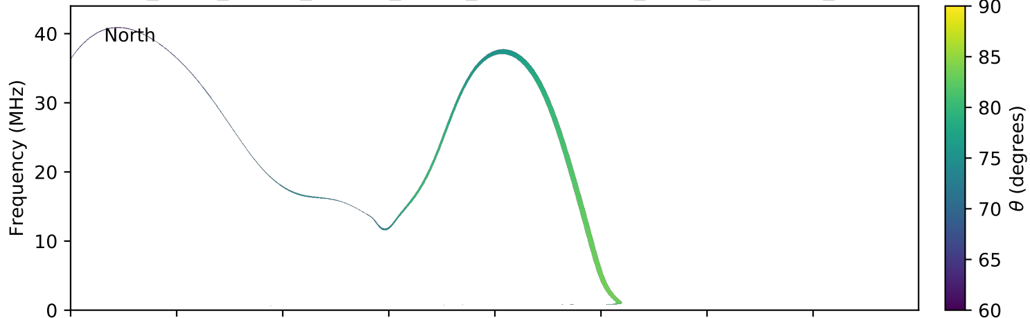
expres_earth_jupiter_europa_jrm09_lossc-wid1deg_3kev_20170613_v01.cdf
