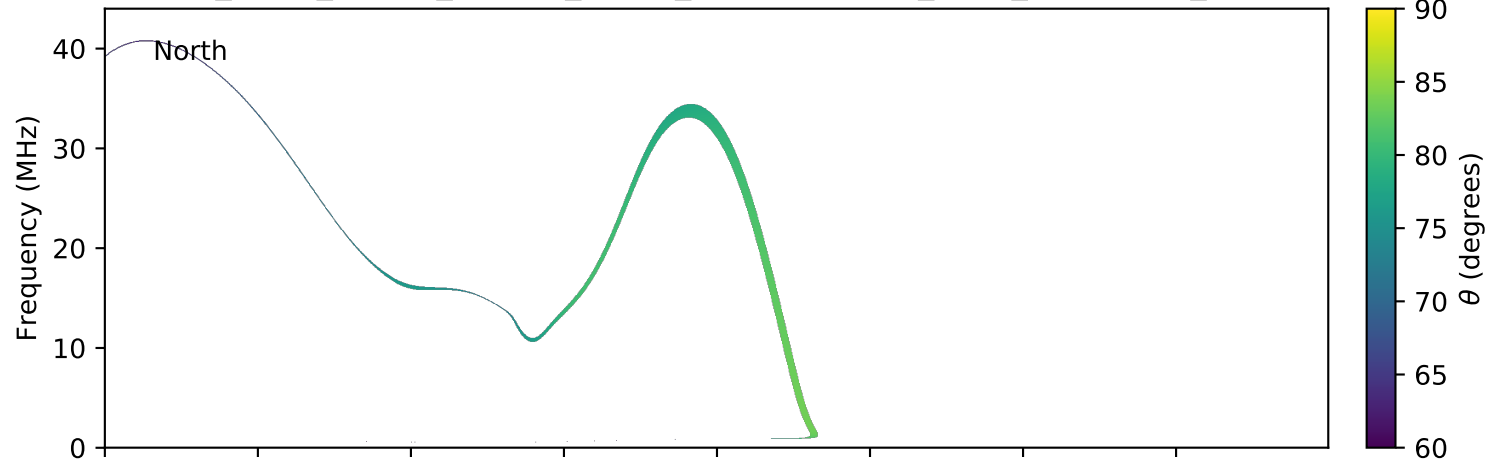
expres_earth_jupiter_europa_jrm09_lossc-wid1deg_3kev_20170606_v01.cdf
