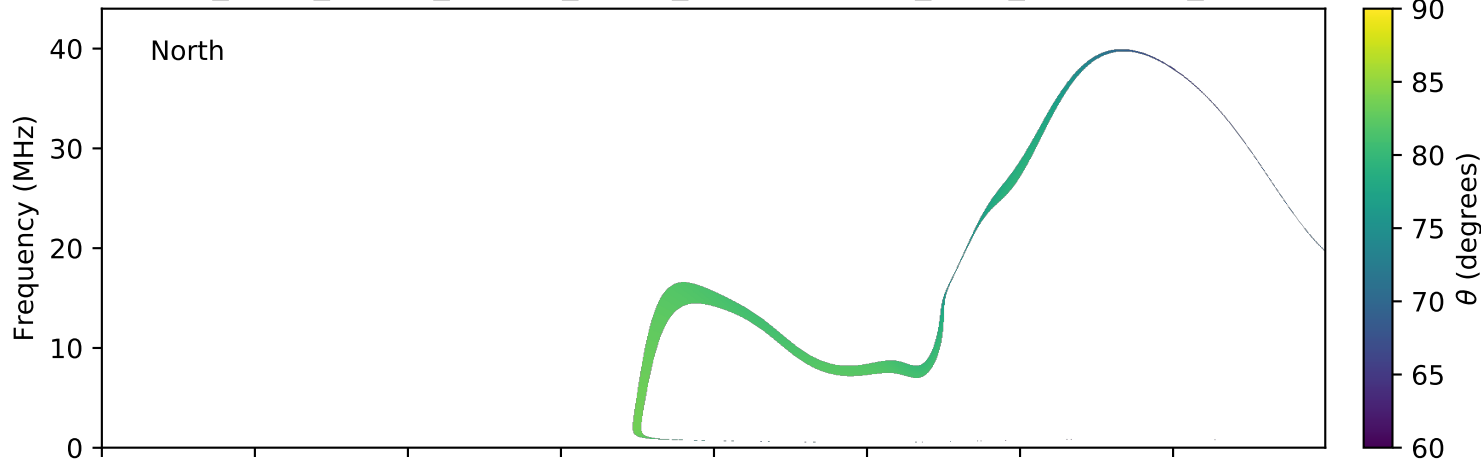
expres_earth_jupiter_europa_jrm09_lossc-wid1deg_3kev_20170601_v01.cdf
