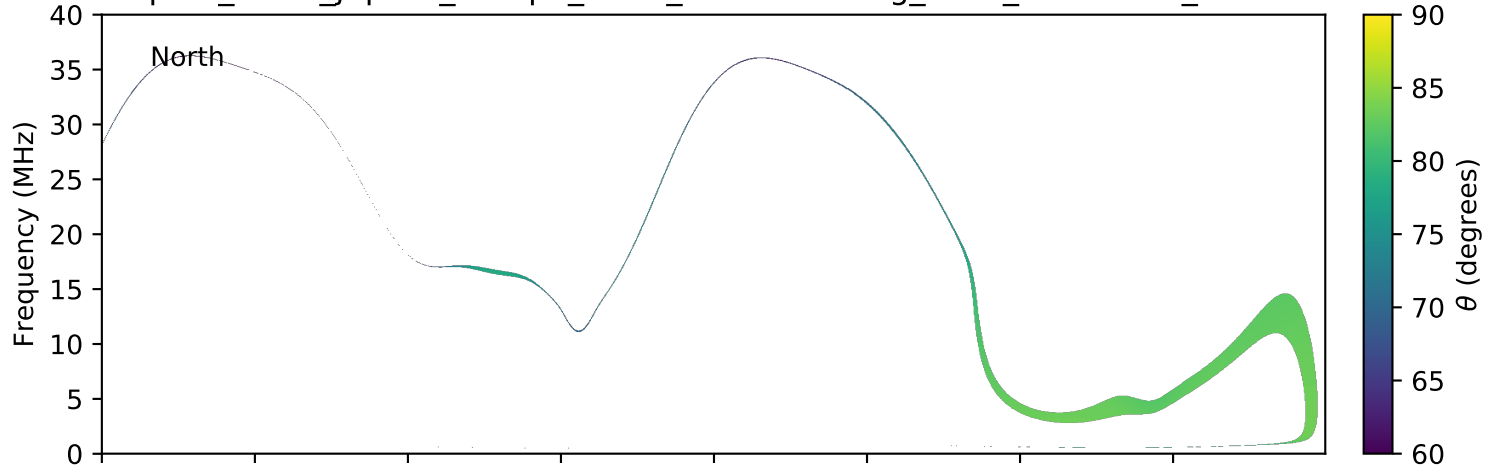
expres_earth_jupiter_europa_isaac_lossc-wid1deg_3kev_20170627_v01.cdf
