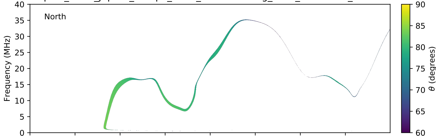
expres_earth_jupiter_europa_isaac_lossc-wid1deg_3kev_20170619_v01.cdf
