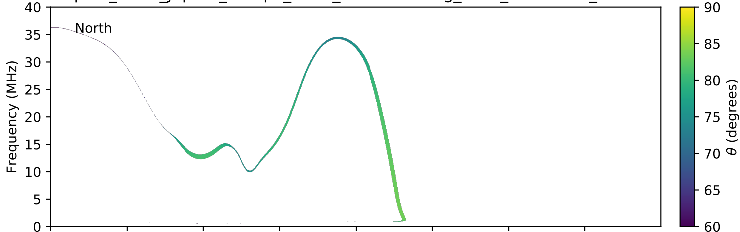
expres_earth_jupiter_europa_isaac_lossc-wid1deg_3kev_20170606_v01.cdf
