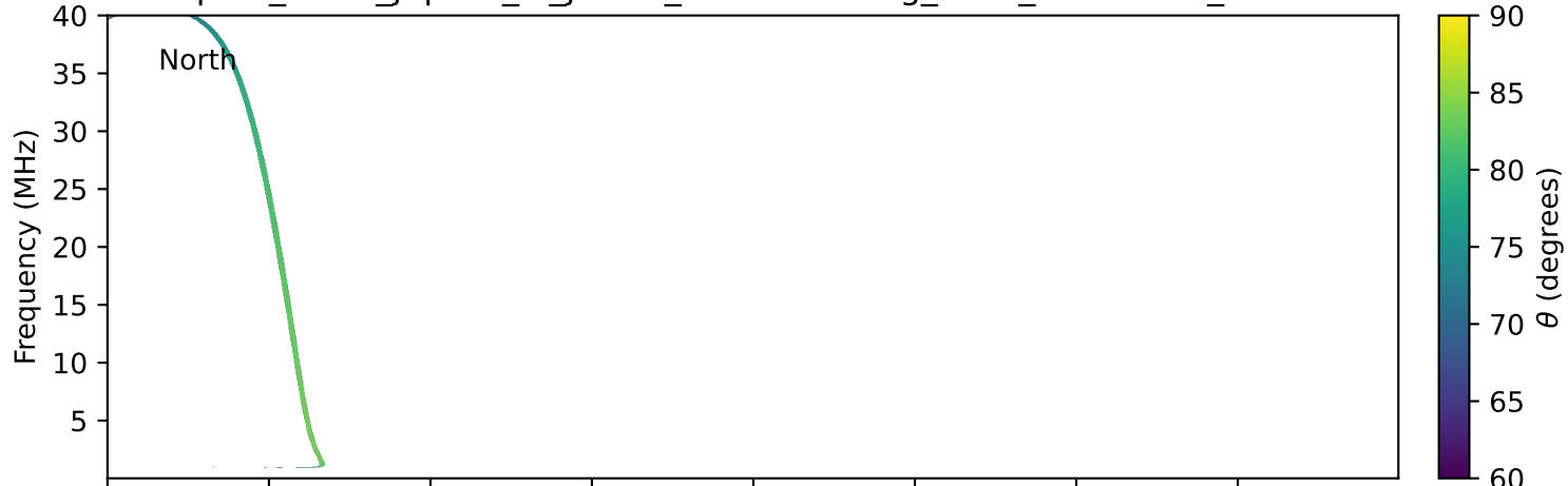
expres_earth_jupiter_io_jrm33_lossc-wid1deg_3kev_20170530_v11.cdf
