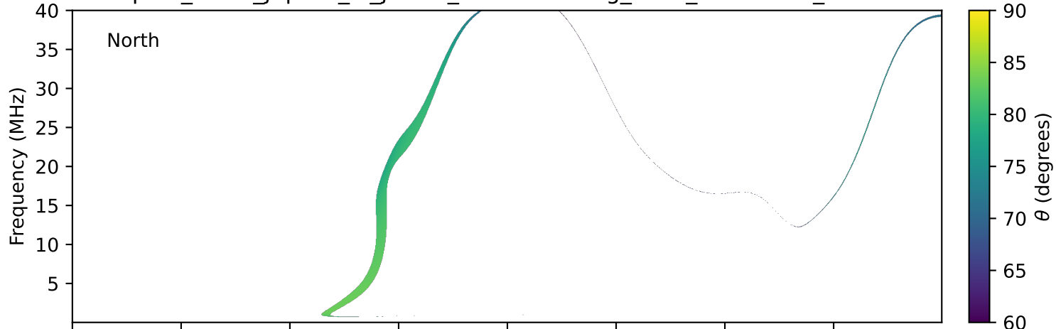
expres_earth_jupiter_io_jrm33_lossc-wid1deg_3kev_20170522_v11.cdf
