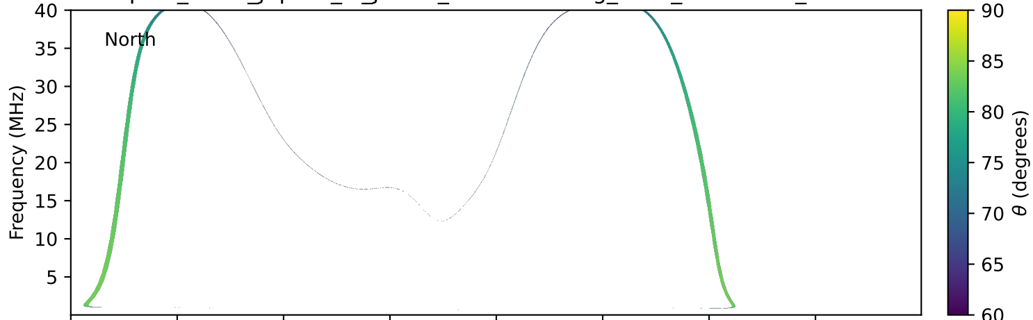
expres_earth_jupiter_io_jrm33_lossc-wid1deg_3kev_20170517_v11.cdf
