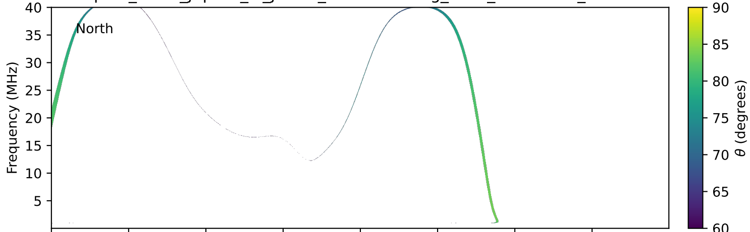
expres_earth_jupiter_io_jrm33_lossc-wid1deg_3kev_20170510_v11.cdf
