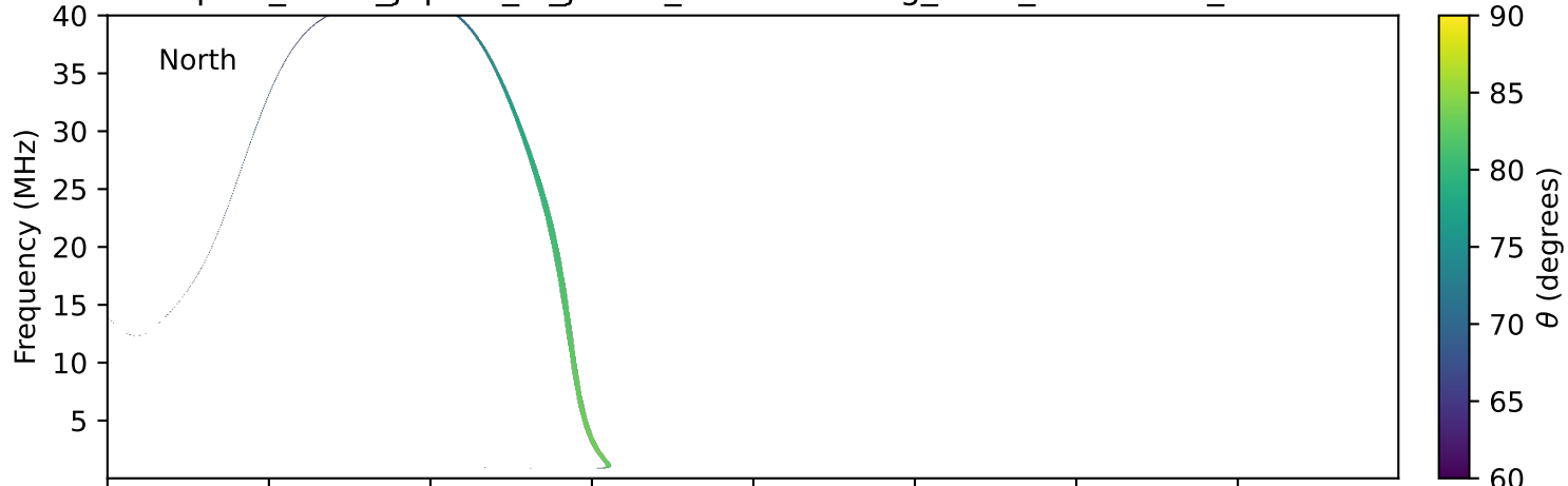
expres_earth_jupiter_io_jrm33_lossc-wid1deg_3kev_20170505_v11.cdf
