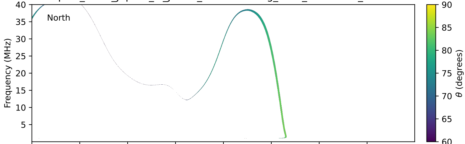
expres_earth_jupiter_io_jrm33_lossc-wid1deg_3kev_20170503_v11.cdf
