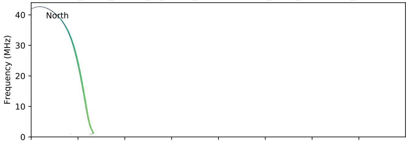
expres_earth_jupiter_io_jrm09_lossc-wid1deg_3kev_20170530_v01.cdf
