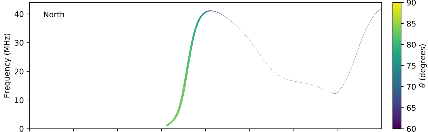
expres_earth_jupiter_io_jrm09_lossc-wid1deg_3kev_20170529_v01.cdf
