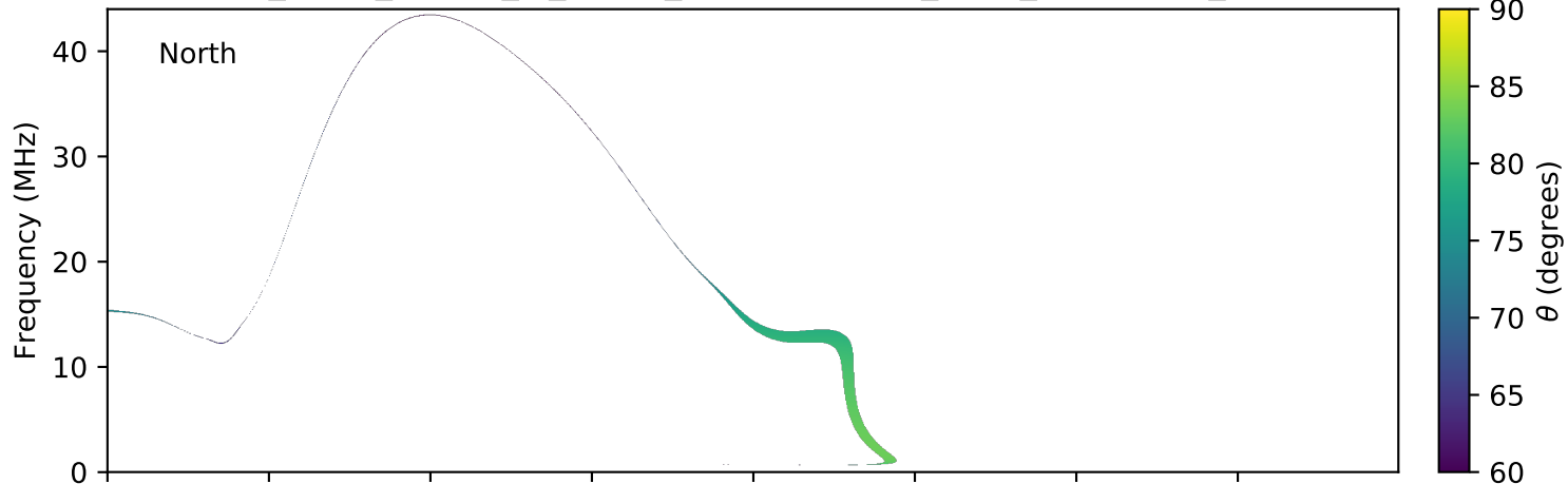
expres_earth_jupiter_io_jrm09_lossc-wid1deg_3kev_20170526_v01.cdf
