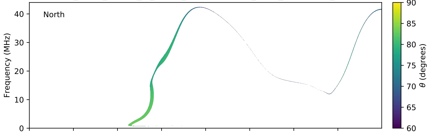
expres_earth_jupiter_io_jrm09_lossc-wid1deg_3kev_20170522_v01.cdf
