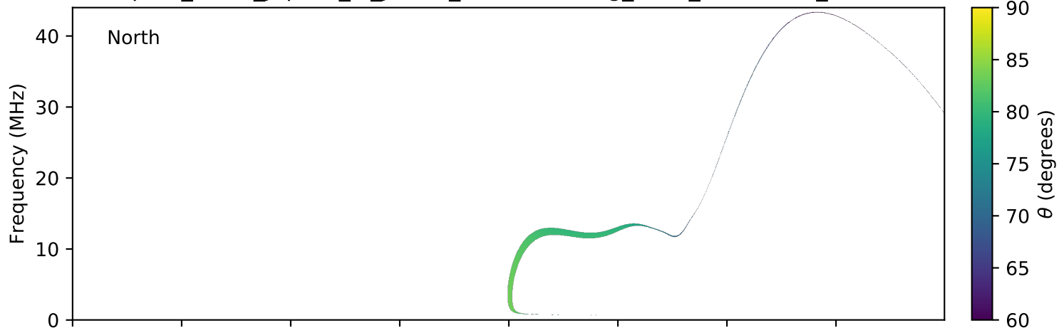
expres_earth_jupiter_io_jrm09_lossc-wid1deg_3kev_20170520_v01.cdf
