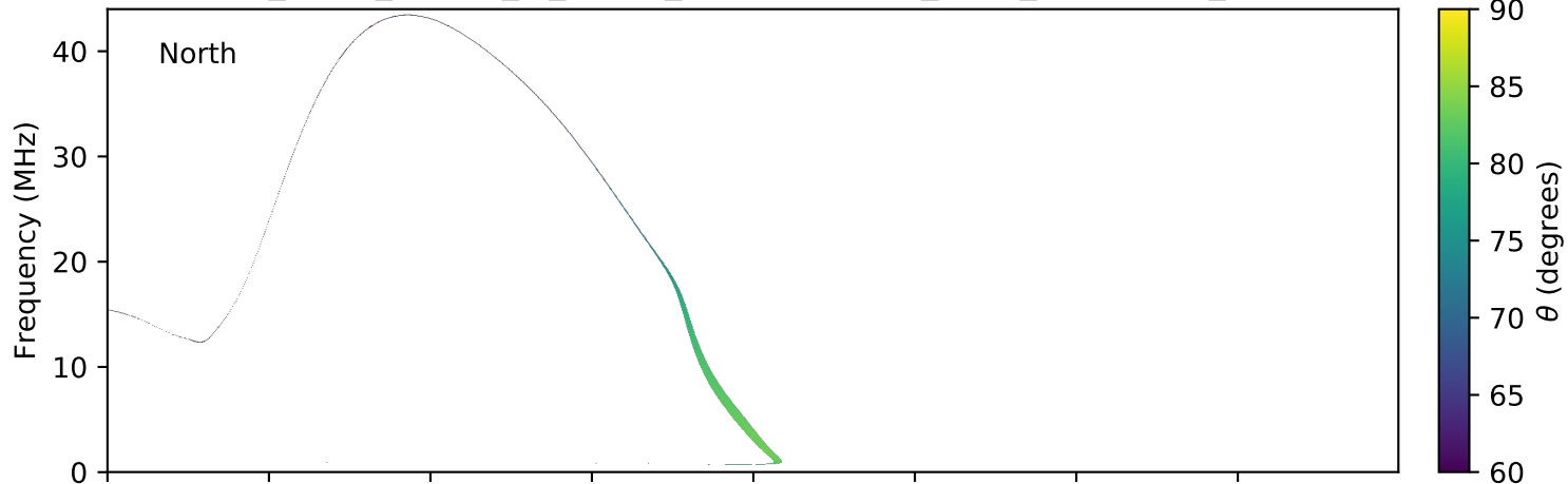
expres_earth_jupiter_io_jrm09_lossc-wid1deg_3kev_20170519_v01.cdf
