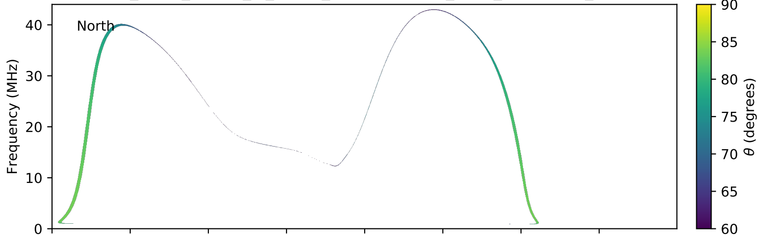
expres_earth_jupiter_io_jrm09_lossc-wid1deg_3kev_20170517_v01.cdf
