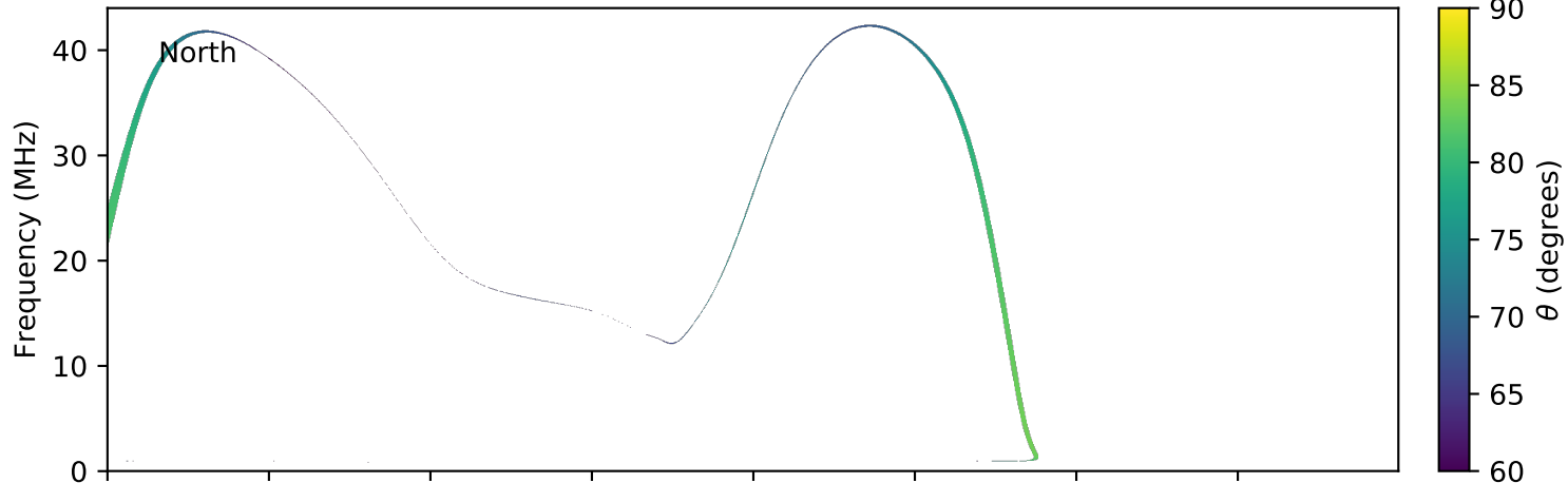
expres_earth_jupiter_io_jrm09_lossc-wid1deg_3kev_20170510_v01.cdf
