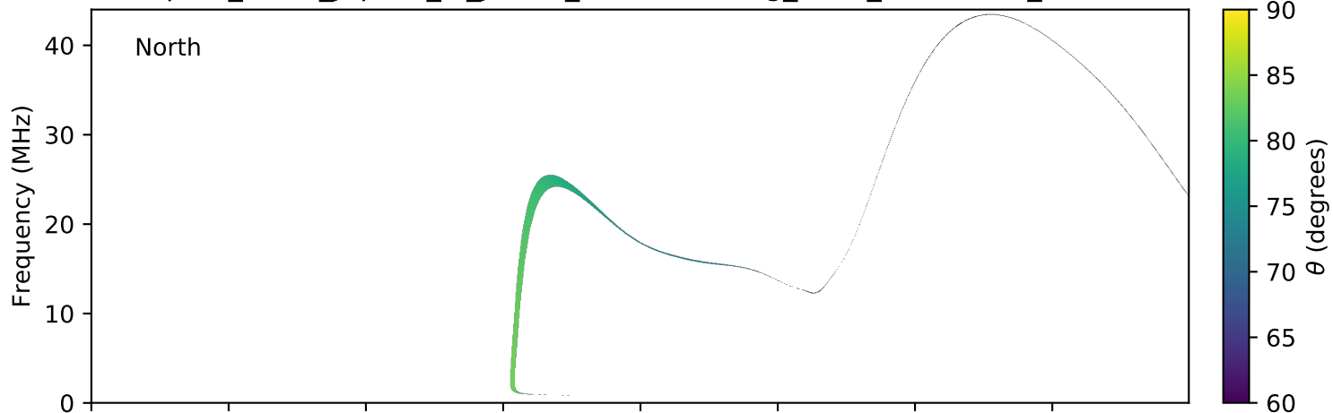
expres_earth_jupiter_io_jrm09_lossc-wid1deg_3kev_20170506_v01.cdf
