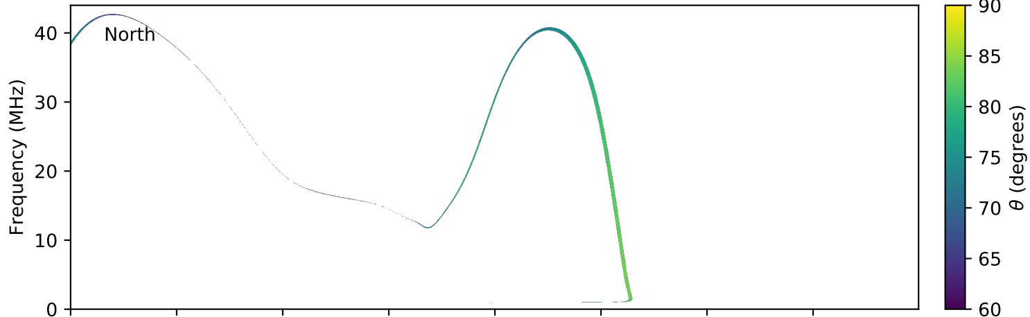
expres_earth_jupiter_io_jrm09_lossc-wid1deg_3kev_20170503_v01.cdf
