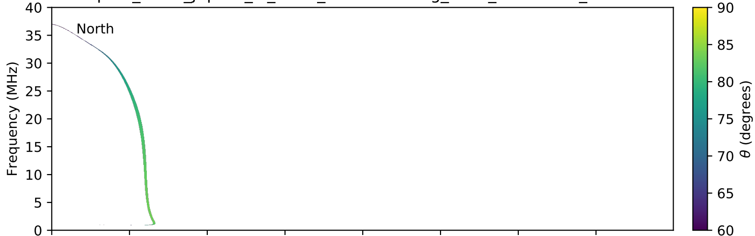
expres_earth_jupiter_io_isaac_lossc-wid1deg_3kev_20170530_v01.cdf
