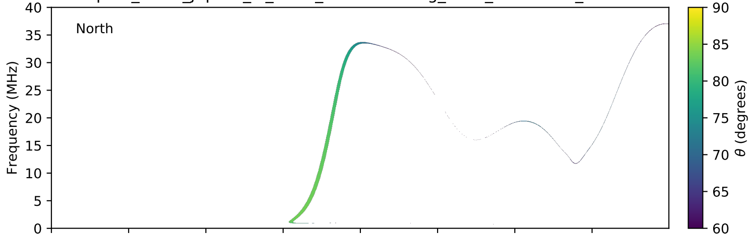
expres_earth_jupiter_io_isaac_lossc-wid1deg_3kev_20170529_v01.cdf
