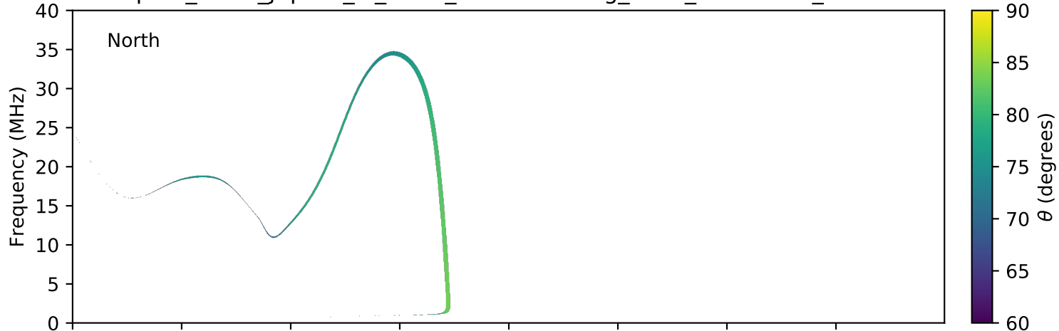
expres_earth_jupiter_io_isaac_lossc-wid1deg_3kev_20170528_v01.cdf
