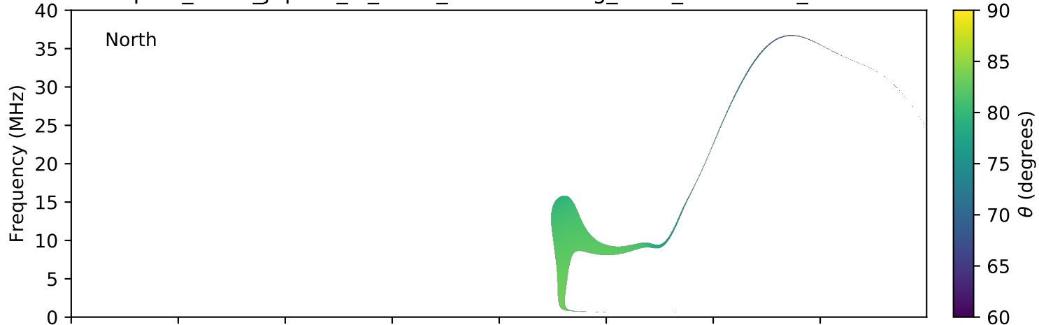
expres_earth_jupiter_io_isaac_lossc-wid1deg_3kev_20170527_v01.cdf
