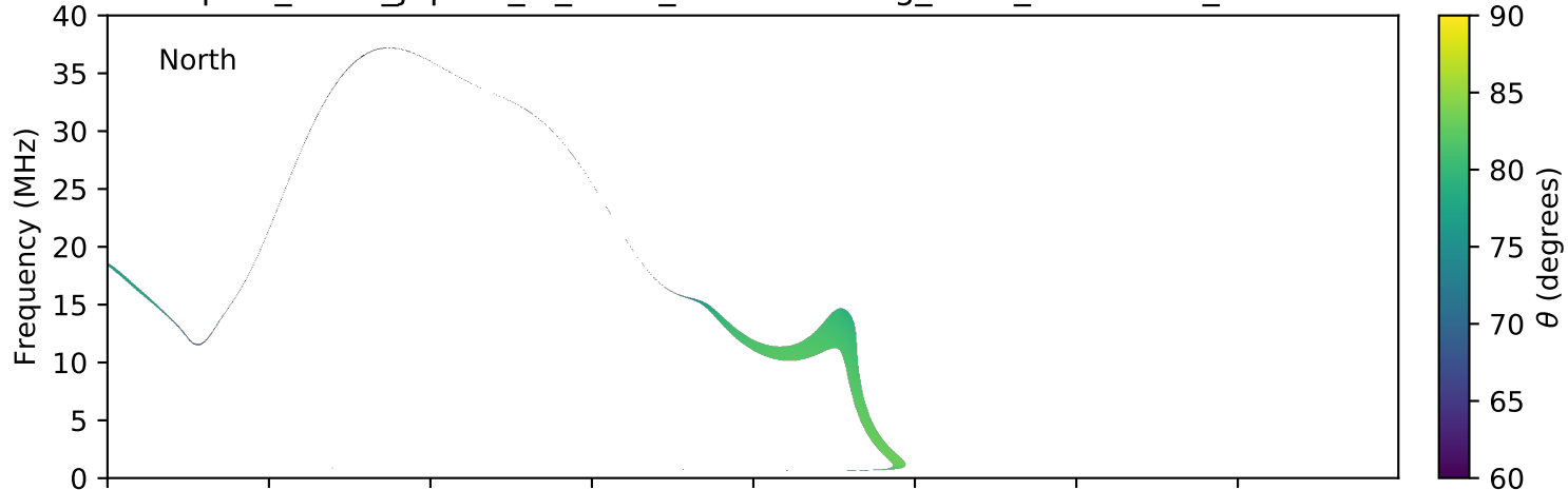
expres_earth_jupiter_io_isaac_lossc-wid1deg_3kev_20170526_v01.cdf
