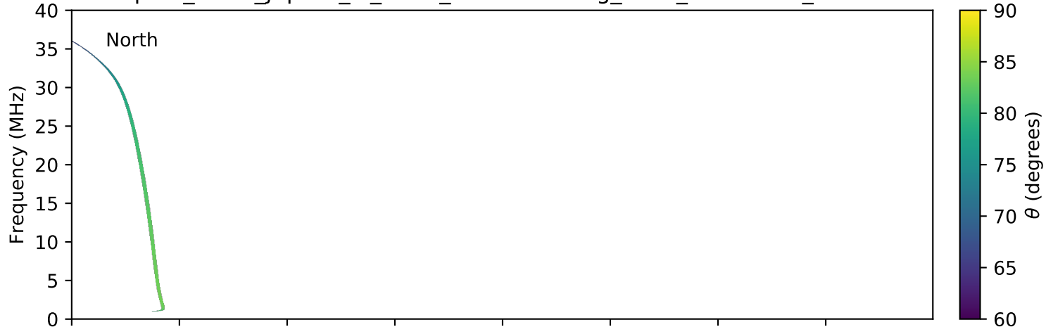
expres_earth_jupiter_io_isaac_lossc-wid1deg_3kev_20170523_v01.cdf
