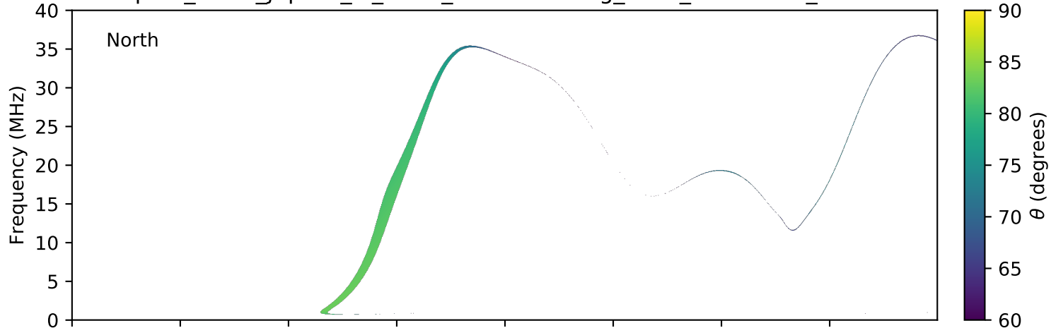
expres_earth_jupiter_io_isaac_lossc-wid1deg_3kev_20170522_v01.cdf
