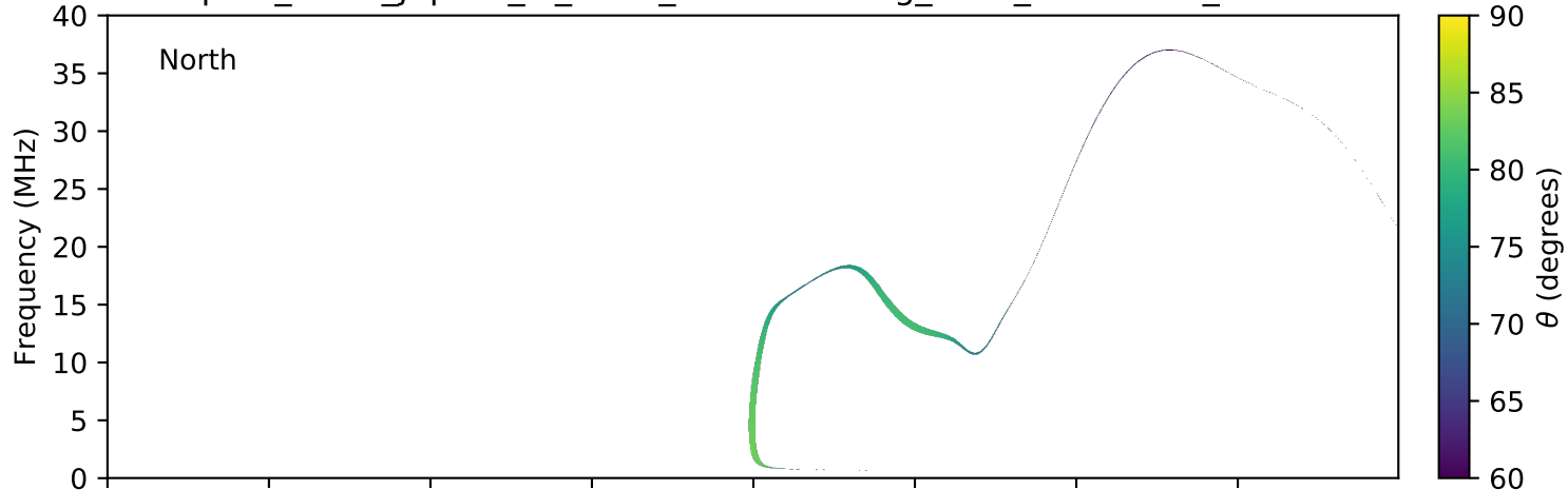
expres_earth_jupiter_io_isaac_lossc-wid1deg_3kev_20170520_v01.cdf
