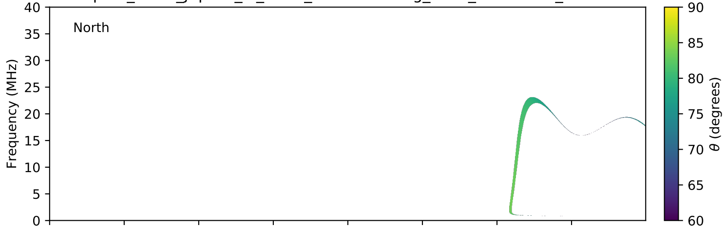
expres_earth_jupiter_io_isaac_lossc-wid1deg_3kev_20170518_v01.cdf
